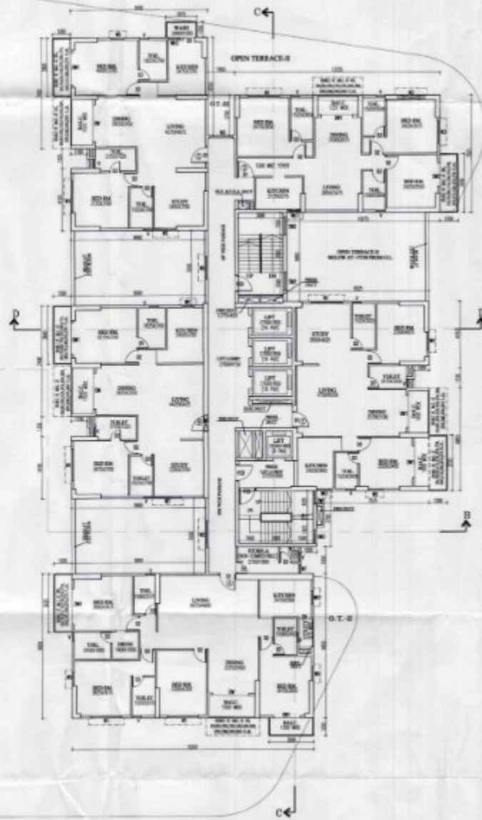
TYPICAL (5TH, 9TH, 11TH, 13TH, 15TH, 19TH & 21ST) FLOOR PLAN TOWER-1
