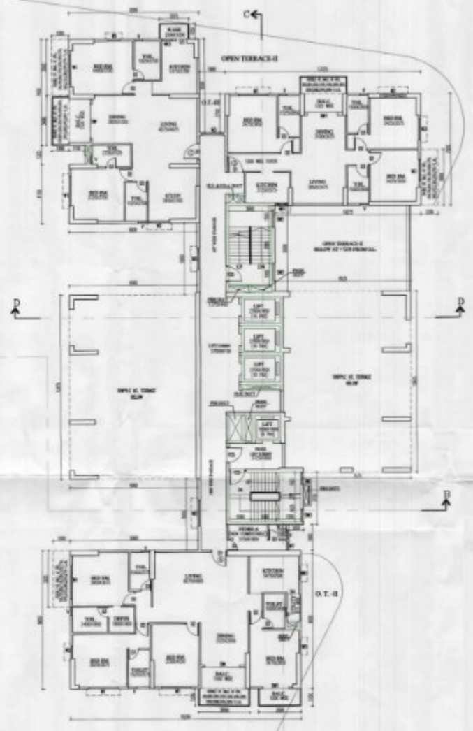
4TH FLOOR PLAN TOWER-1
