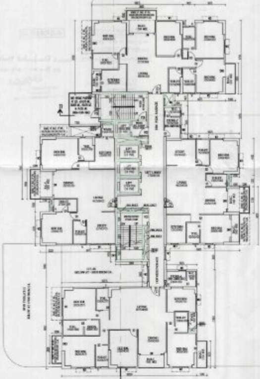
12TH FLOOR PLAN TOWER-2
